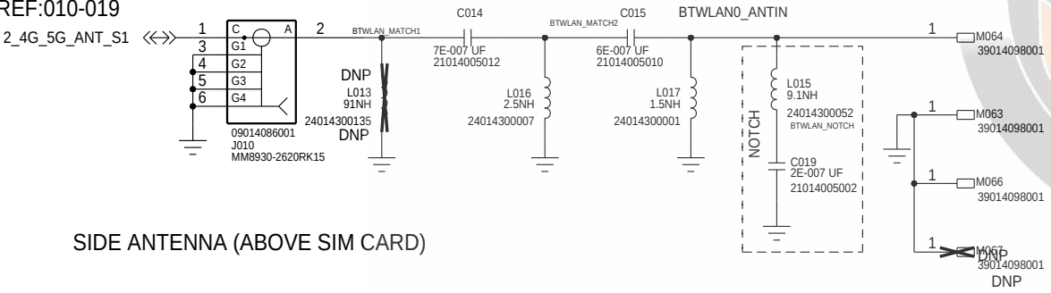
BT/WLAN CHAIN0 ANTENNA REF:010-019
