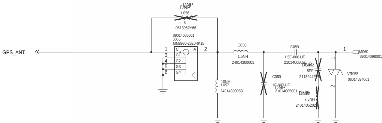
GPS ANTENNA REF: 055-069
